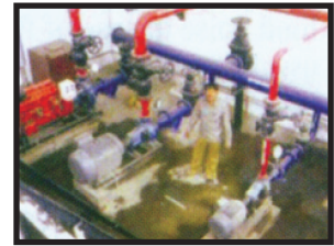
Positive Pressure Fire Pump House
